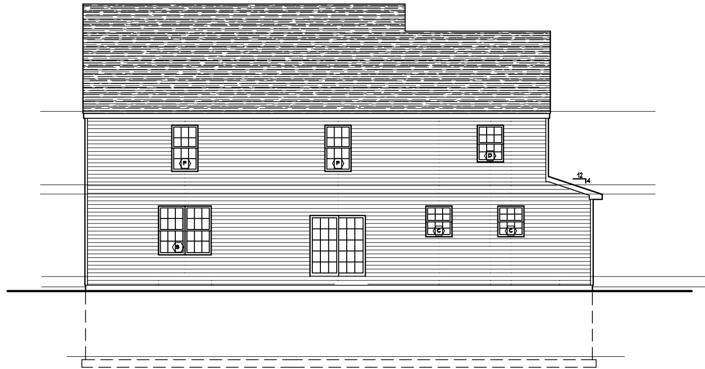
REAR ELEVATION
