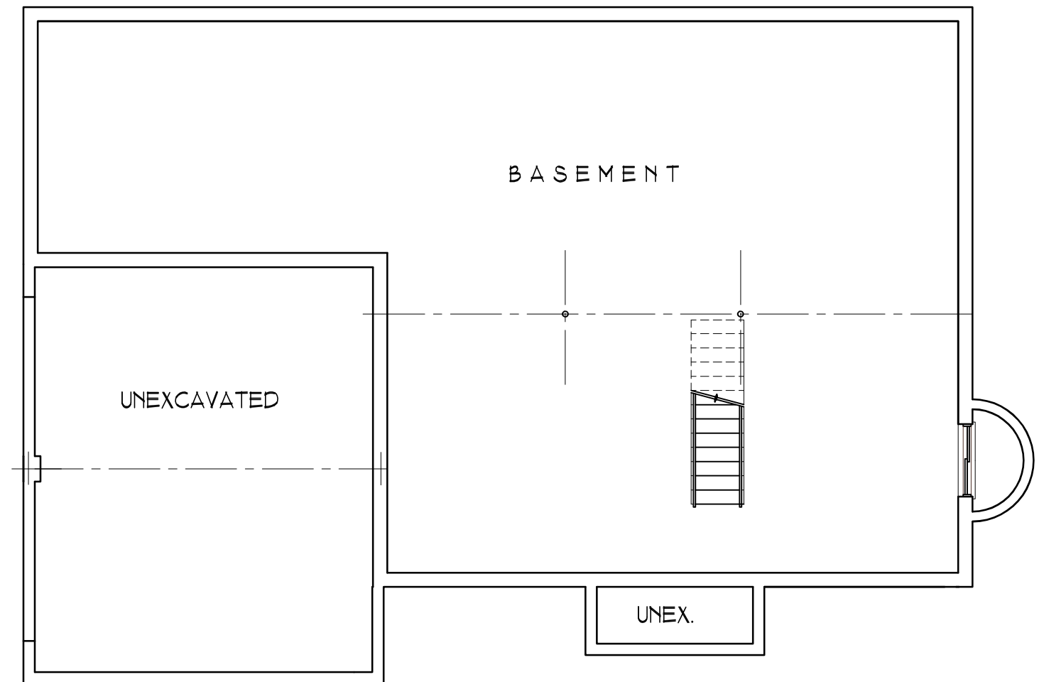
BASEMENT PLAN
